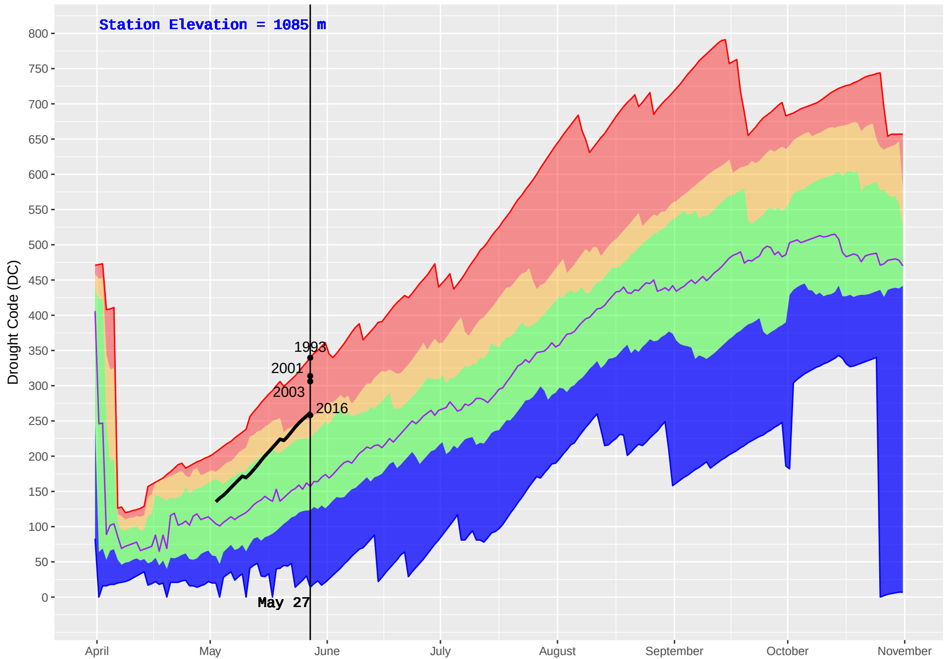
TAUTRI (206) : Historical (1970–2016) and Current (2018) Noon Drought Code (DC)
