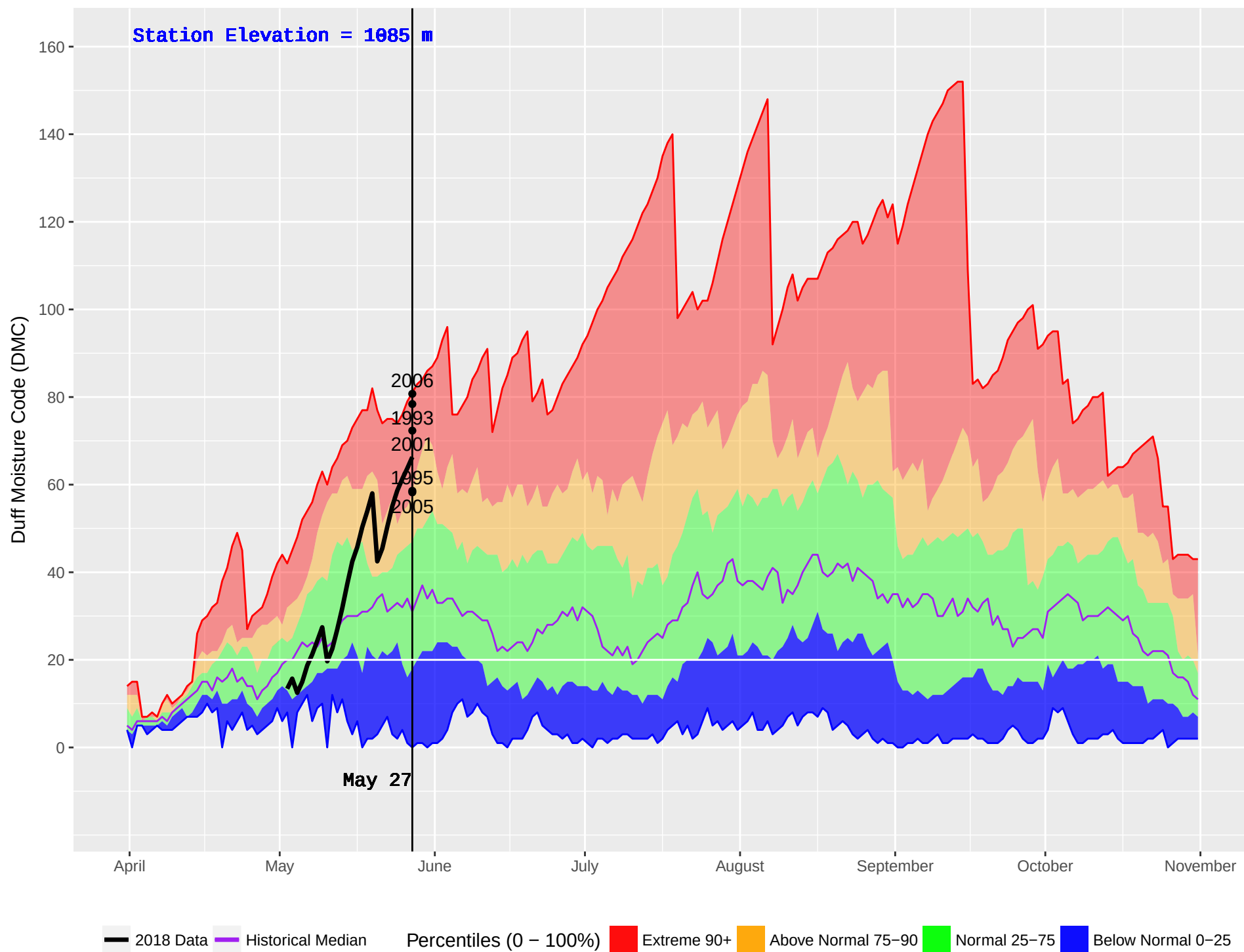
TAUTRI (206) : Historical (1970–2016) and Current (2018) Noon Duff Moisture Code (DMC)
